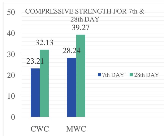
Graph 3: Graphical representation of combined compressive strength for 7 th and 28 th day.
