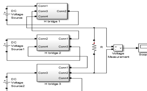
Fig 8: Simulation model of seven level inverter
