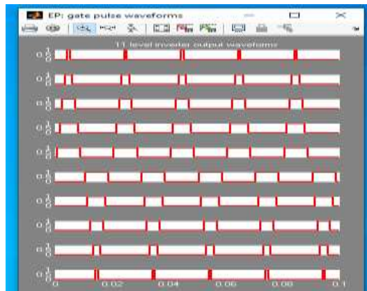
Fig 13(a1): Gate pulse for eleven level inverter: EPPWM
