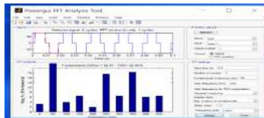
Fig 10(b1): THD waveforms of three level inverter: EPPWM
