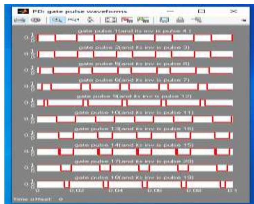
Fig 13(a2): Gate pulse for eleven level inverter: PDPWM
