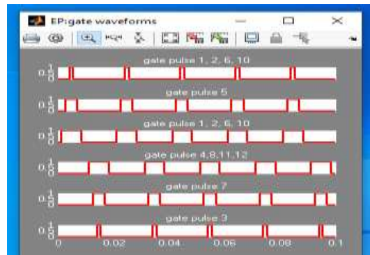
Fig 12(a1): Gate pulse for seven level inverter: EPPWM
