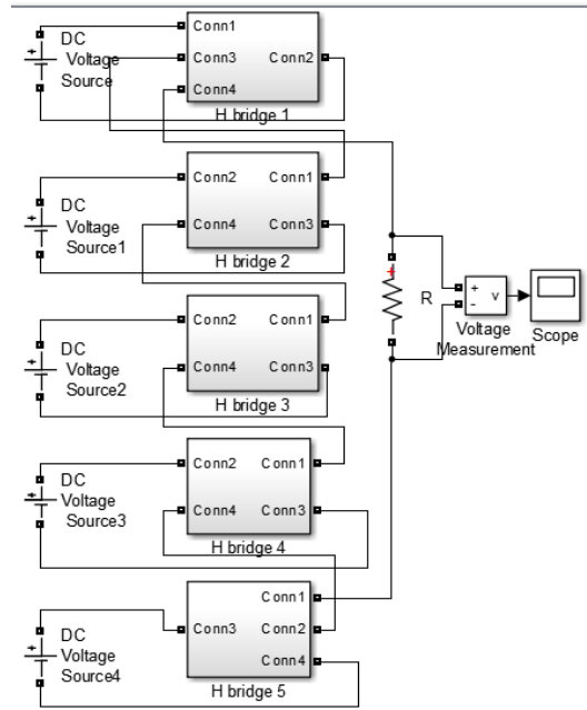
Fig 9: Simulation model of eleven level inverter
