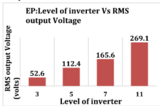
Fig 15: Graph of level of inverter vs RMS output voltage for EPPWM
