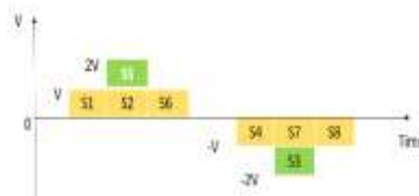
Fig 5: Switching pattern of five level Inverter using EP-PWM
