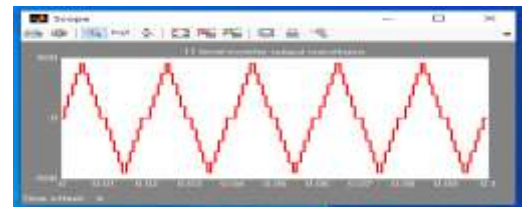
Fig 13(c): Eleven level Output waveform
