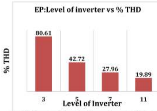
Fig 14: Graph of level of inverter vs %THD and for EPPWM
