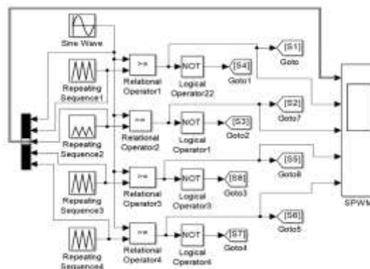
Fig 3: Generation of multi-carrier signal (SPWM) (Five level)
