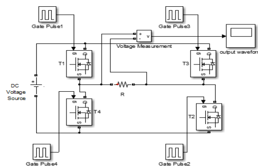
Fig 6: Simulation model of three level inverter
