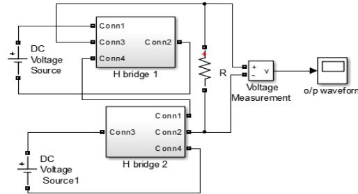
Fig 7: Simulation model of Five level inverter
