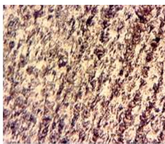
Material Grade-IS 2062 E350C/HT-50 (As Rolled Ferrite & Ferrite) @100X
