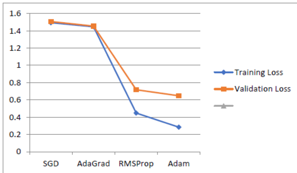
Comparison Graph between Optimizers
