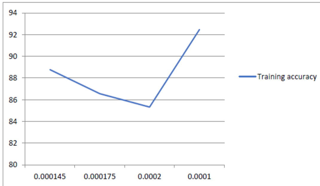
Learning Rate vs Training Accuracy for Adam Optimizer
