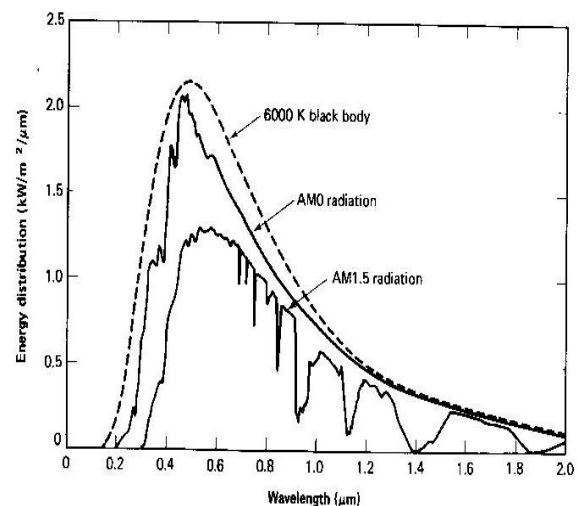
Figure (2) Spectral distribution of sunlight [3].
