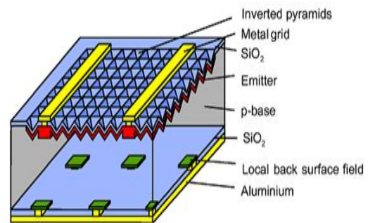
Figure (4) Structure of a high-efficiency monocrystalline solar cell [4].
