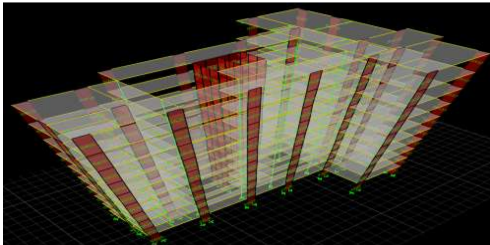
Fig.no.8: 3DviewofG+9 RC T-shape building.
