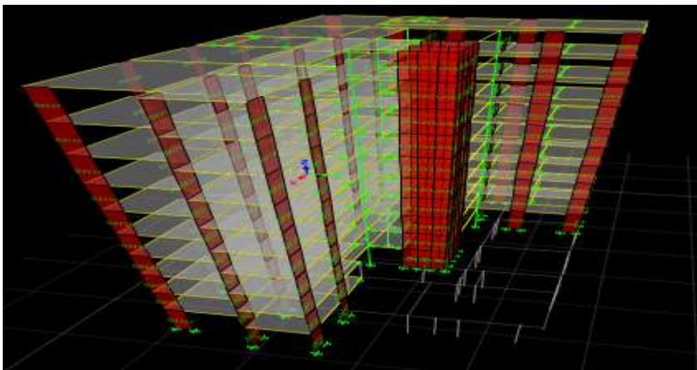
Fig.no.6: 3DviewofG+9 RC L-shape building.
