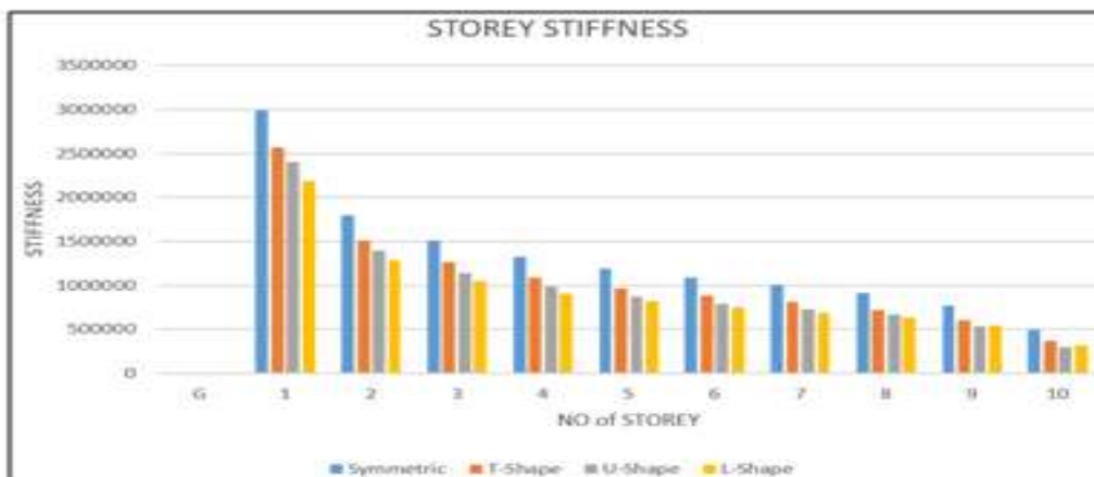
Fig.no.10: Graph of Storey Stiffness
