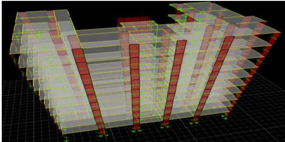
Fig.no.7: 3DviewofG+9 RC U-shape building.
