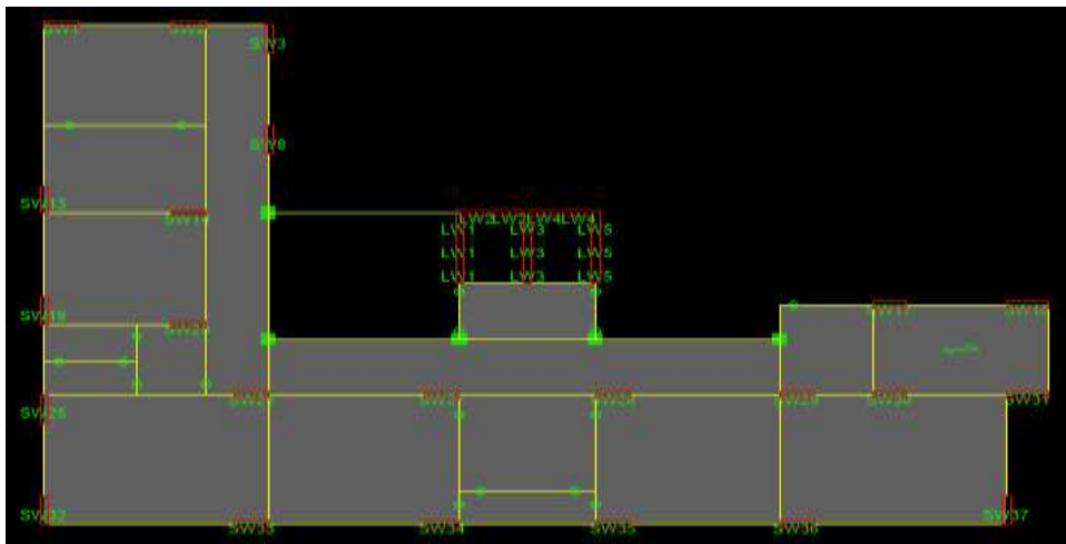
Fig.no.2: Planview of G+9 RC
