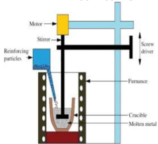
Fig.2.1 Stir casting process setup
