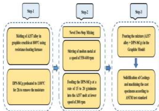
Fig.2.2 Flowchart of fabrication process
