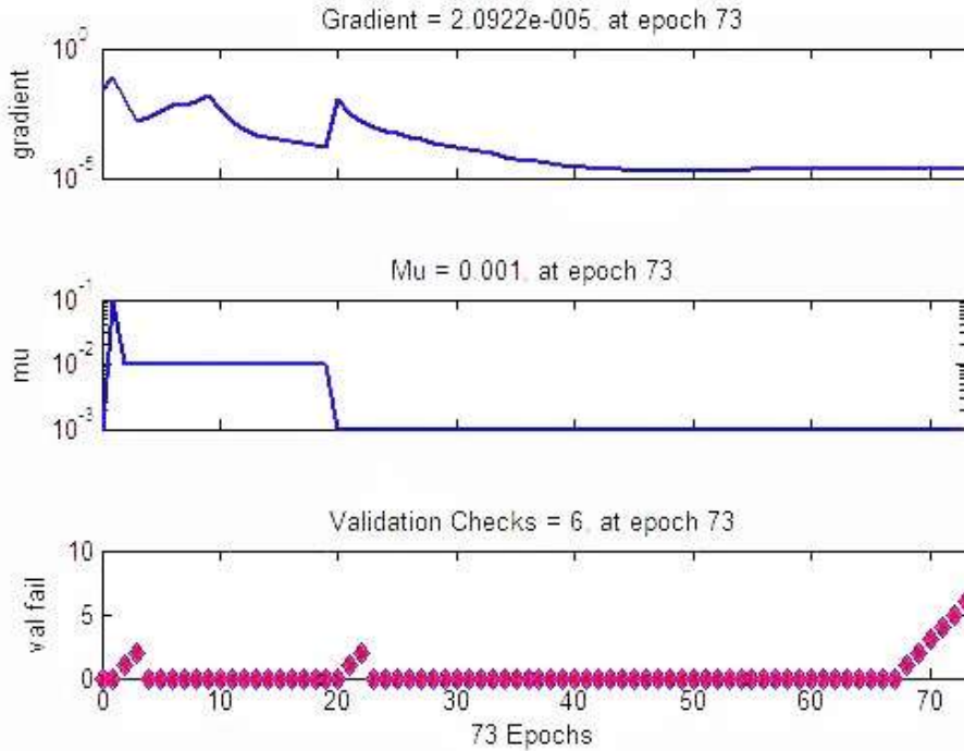
Figure 4 Plottrainstate
