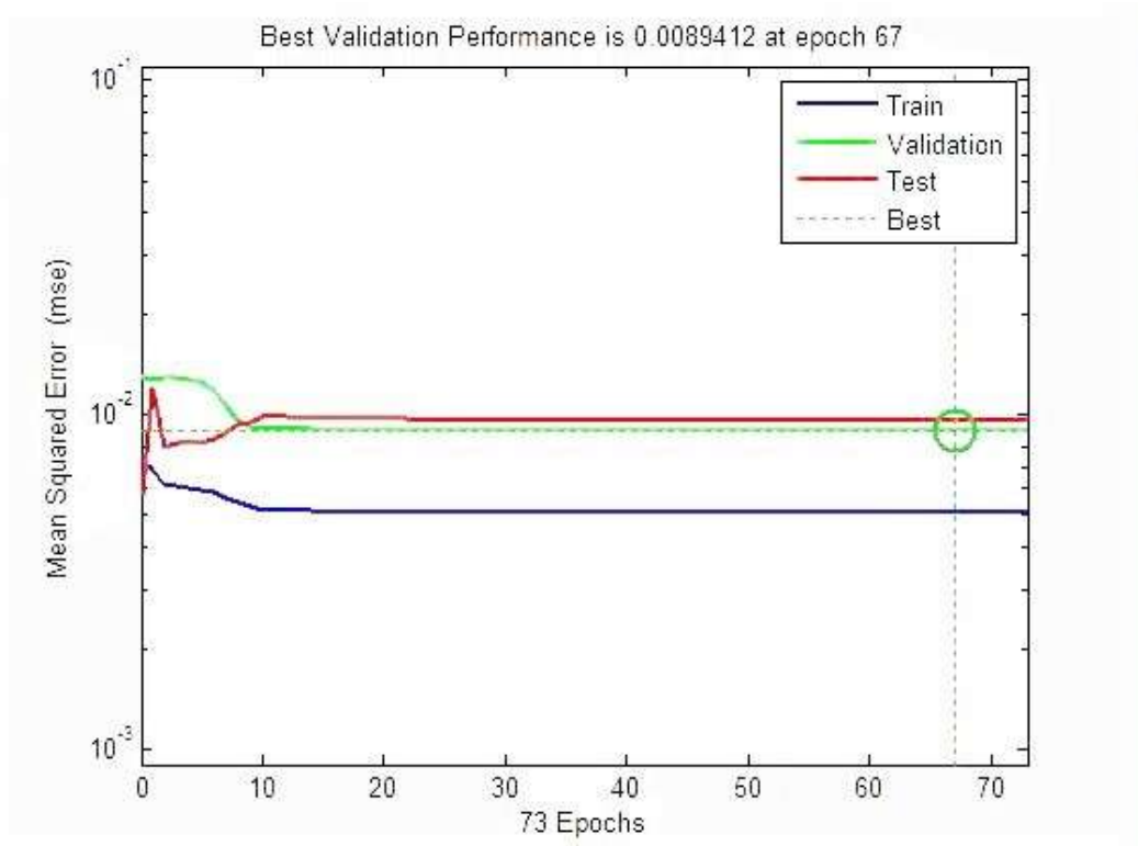
Figure 3. Plotperform
