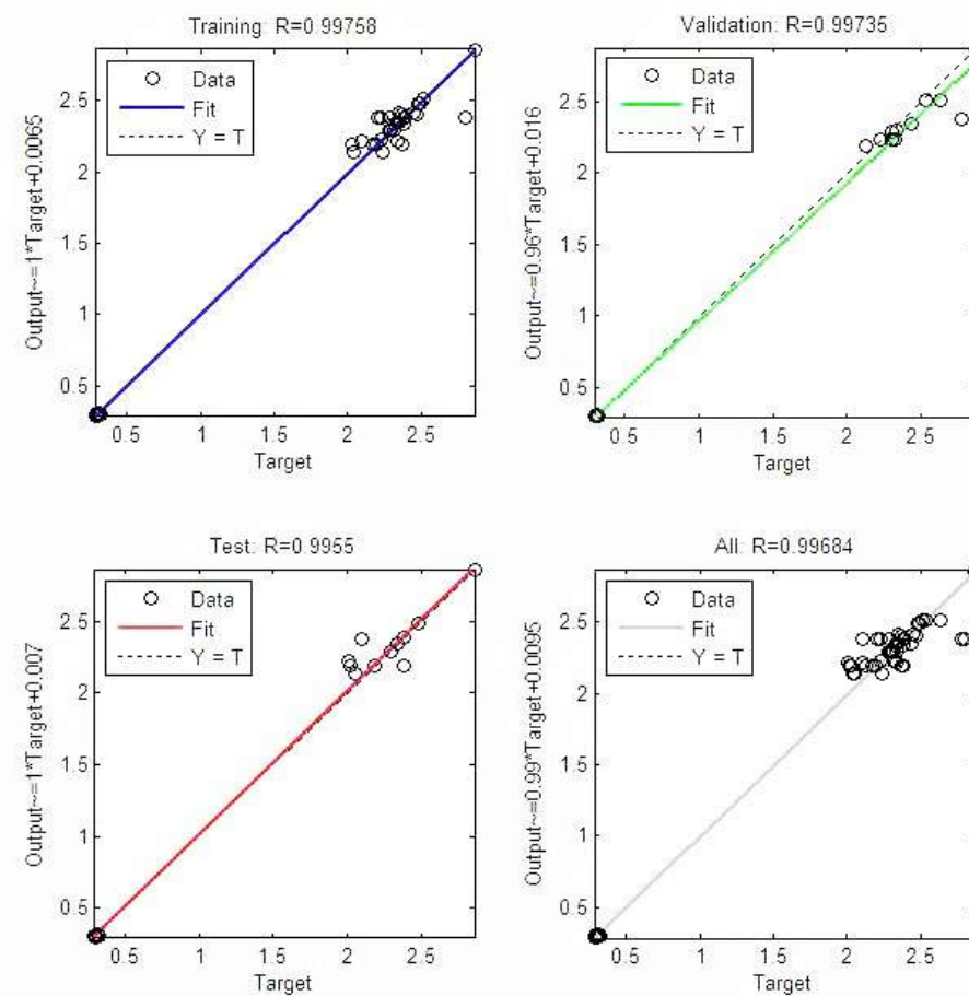
Figure 5. plotregression
