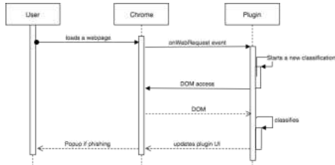
Fig-2: Working Sequence Diagram
