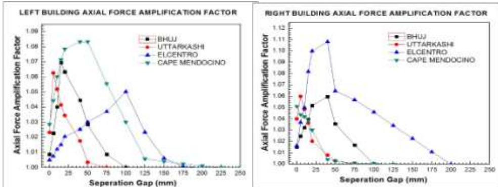
Graph 3-Axial force amplification factor versus gap for slab to slab pounding
