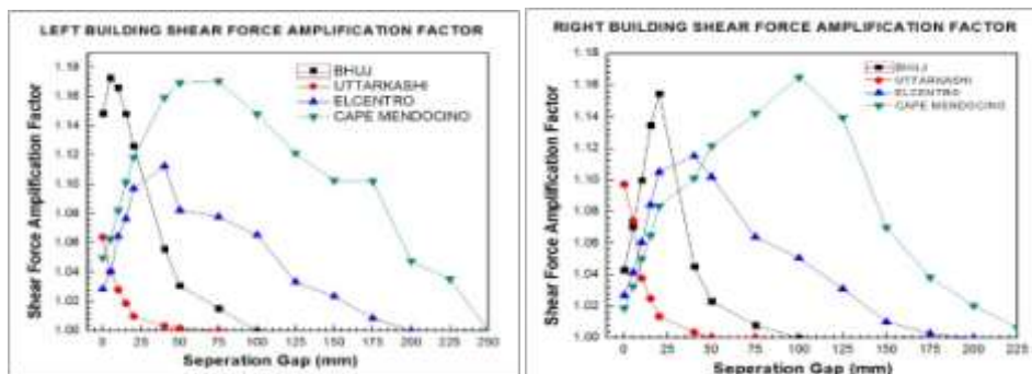
Graph 5- Shear force amplification factor versus gap for slab to slab pounding
