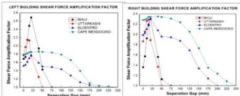
Graph 6-Shear force amplification factor versus gap for mid column pounding
