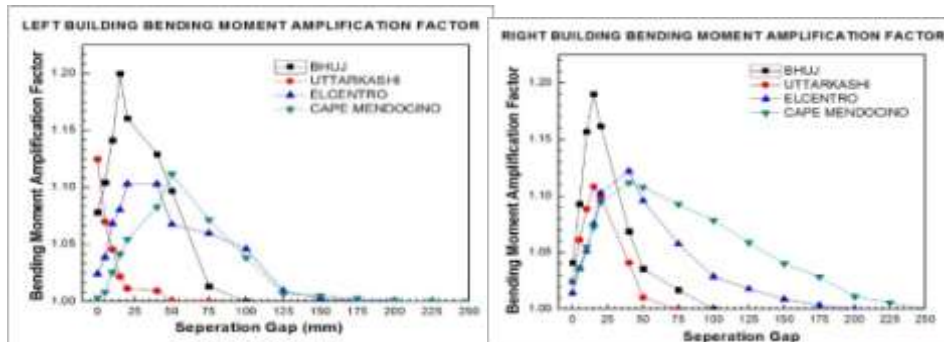
Graph 7-Bending moment amplification factor versus gap for slab to slab pounding
