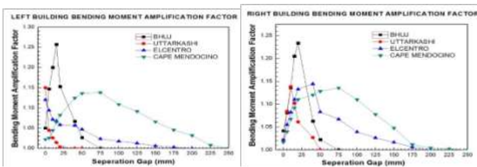
Graph 8- Bending moment amplification factor versus gap for mid column pounding
