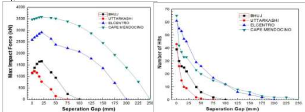
Graph 1- Maximum Pounding force and number of hits versus gap for slab to slab pounding
