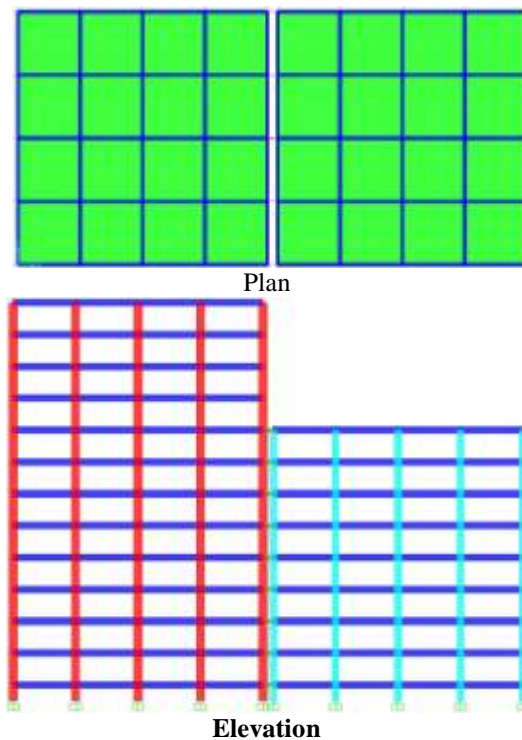
Fig. 1 Plan and elevation of buildings considered for slab to slab pounding
