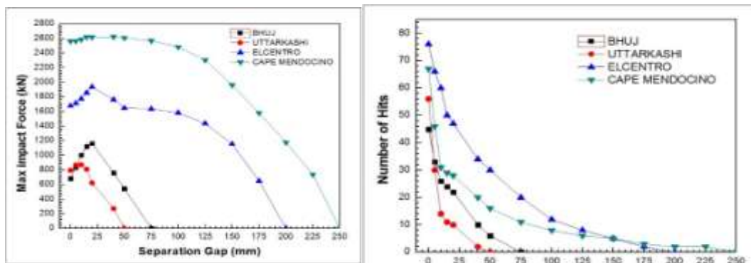
Graph 2- Maximum Pounding force and number of hits versus gap for mid column pounding
