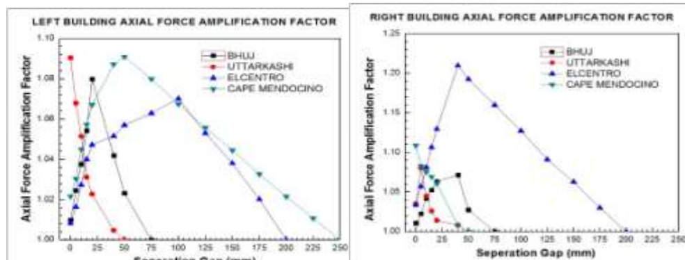
Graph 4- Axial force amplification factor versus gap for mid column pounding
