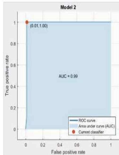
Fig. (7). ROC Curve
