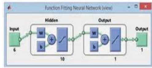
Fig.(3).AppliedNeuralNetworkModel
