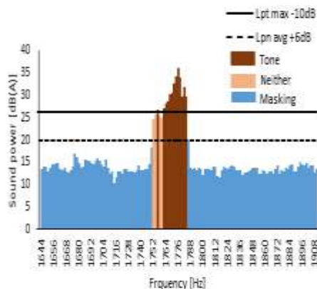
Figure 7: Classification of spectral lines
