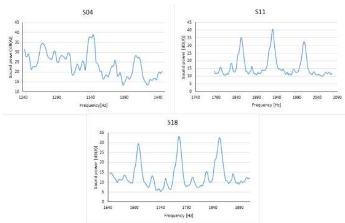
Figure 8: Critical bandwidth of spectra S04, S11, and S18
