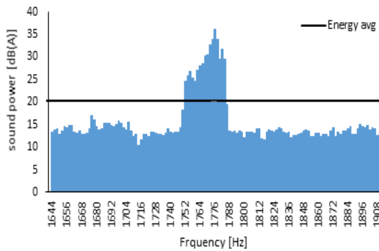
Figure 4: Energy average of spectrum S01
