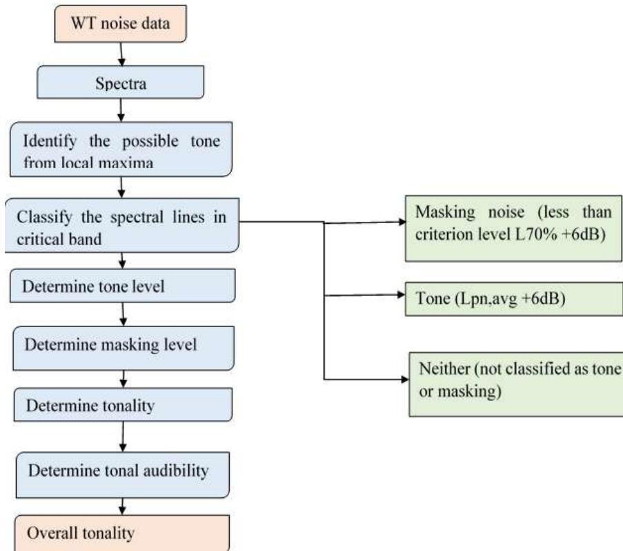
Figure 1: Tonality analysis methodology
