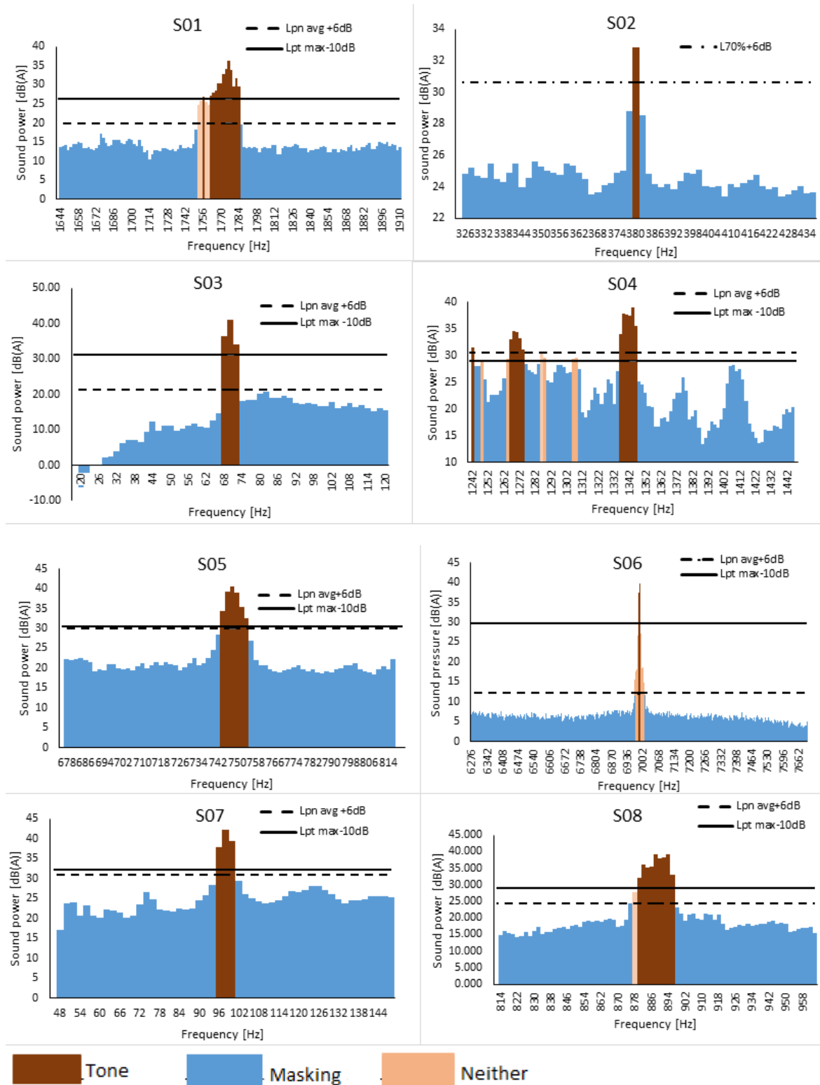
Figure 9: Classification of the spectral line for all spectra
