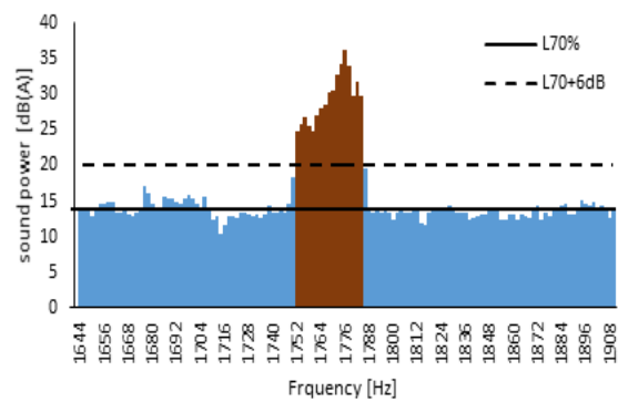
Figure 5: L70% energy average of S01
