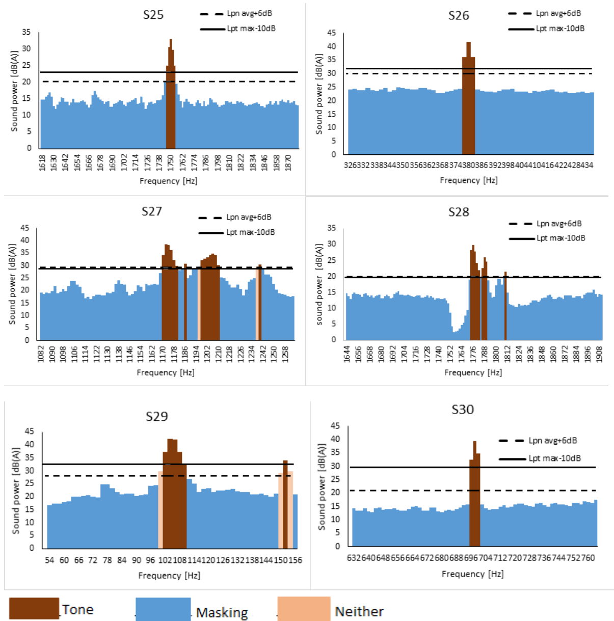
Figure 9: Classification of the spectral line for all spectra(continuation) Note: S- Sample spectra, S02 and S13 have no identified tone hence L70%+6dB is taken
