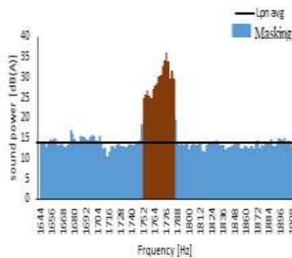
Figure 6: Masking noise level of S01
