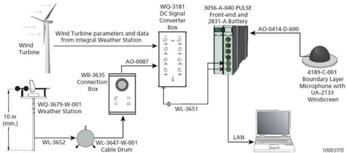
Figure 2: Typical wind turbine noise measurement setup [16]
