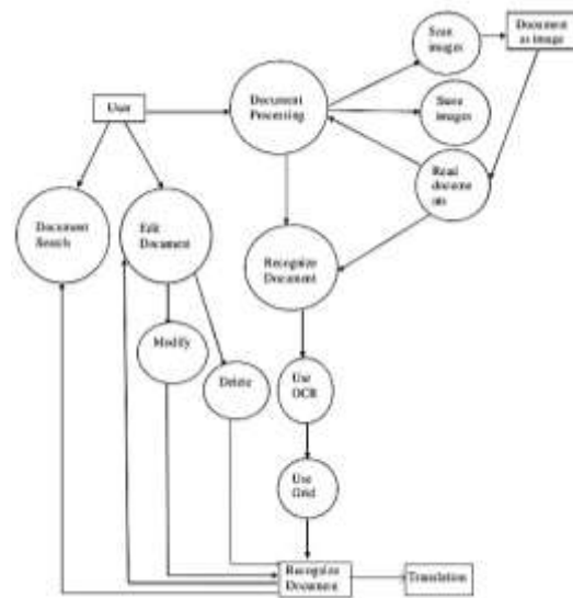
Fig 3: Dataflow Diagram
