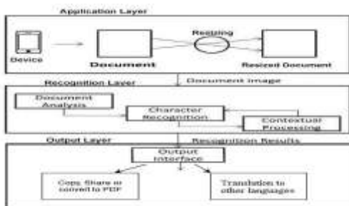
Fig 2: System Architecture
