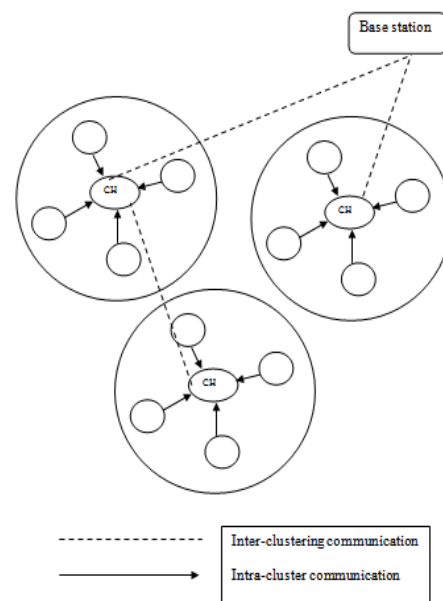
Fig.1 Types of data transfer in clustered networks.
