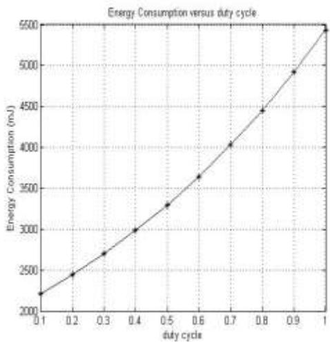
Fig.5 Energy Consumption versus duty cycle for r=80
