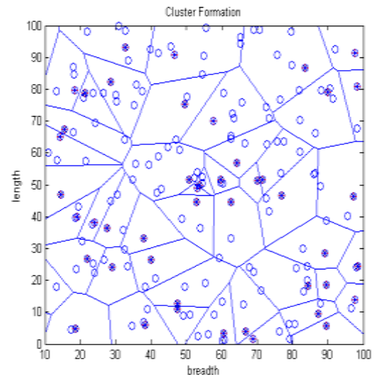
Fig.2 Initial Clustering
