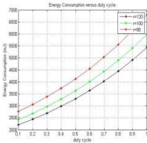
Fig.8 Energy Consumption versus duty cycle for variations in values of r
