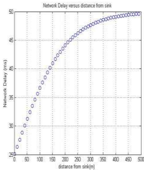
Fig.9 Network Delay versus distance from sink
