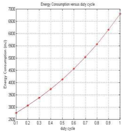
Fig.7 Energy Consumption versus duty cycle for r=120
