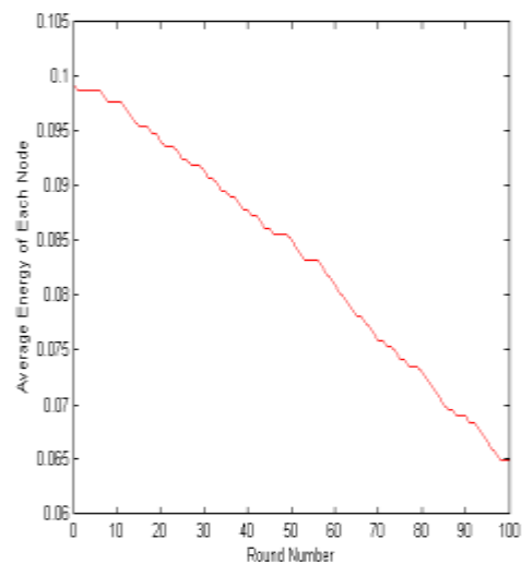
Fig.3 Average Energy of Nodes
