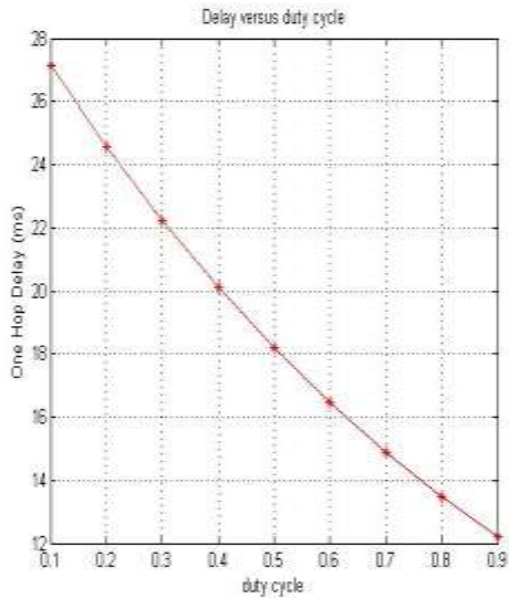
Fig.4 One hop Delay versus duty cycle
