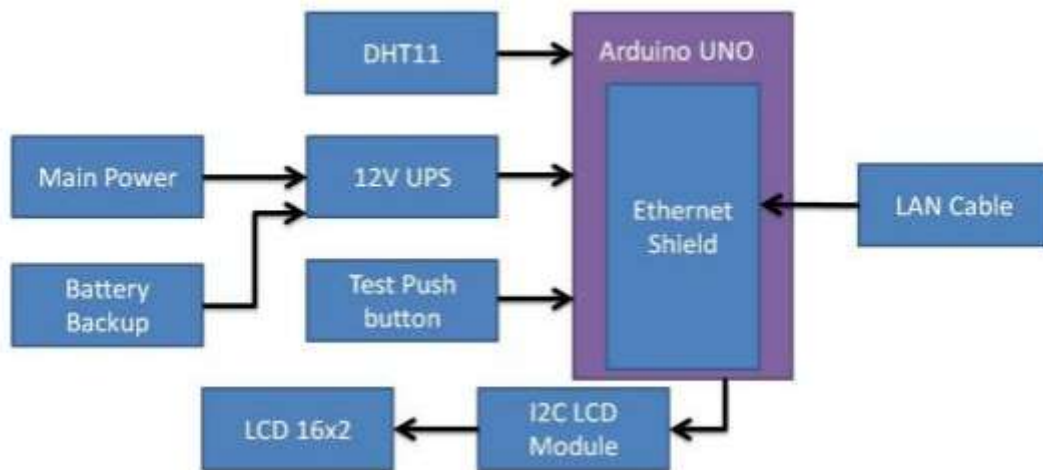
Fig. BLOCK DIAGRAM OF TRANSMITTER DEVICE
