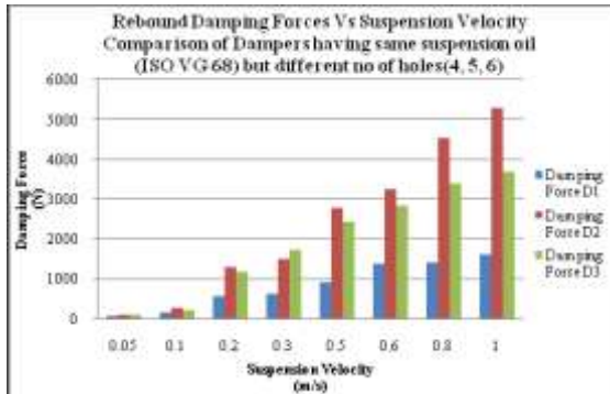
Fig.6 Comparison of all the dampers for Damping Forces in Rebound stroke
