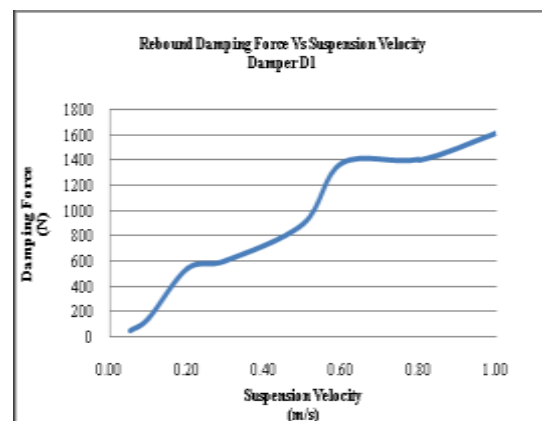
Fig.5 Rebound Damping Force Vs Suspension Velocity
