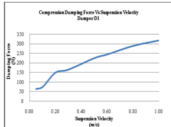
Fig.4 Compression Damping Force Vs Suspension Velocity
