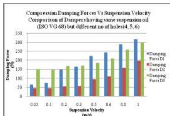
Fig.6 Comparison of all the dampers for Damping Forces in Compression stroke
