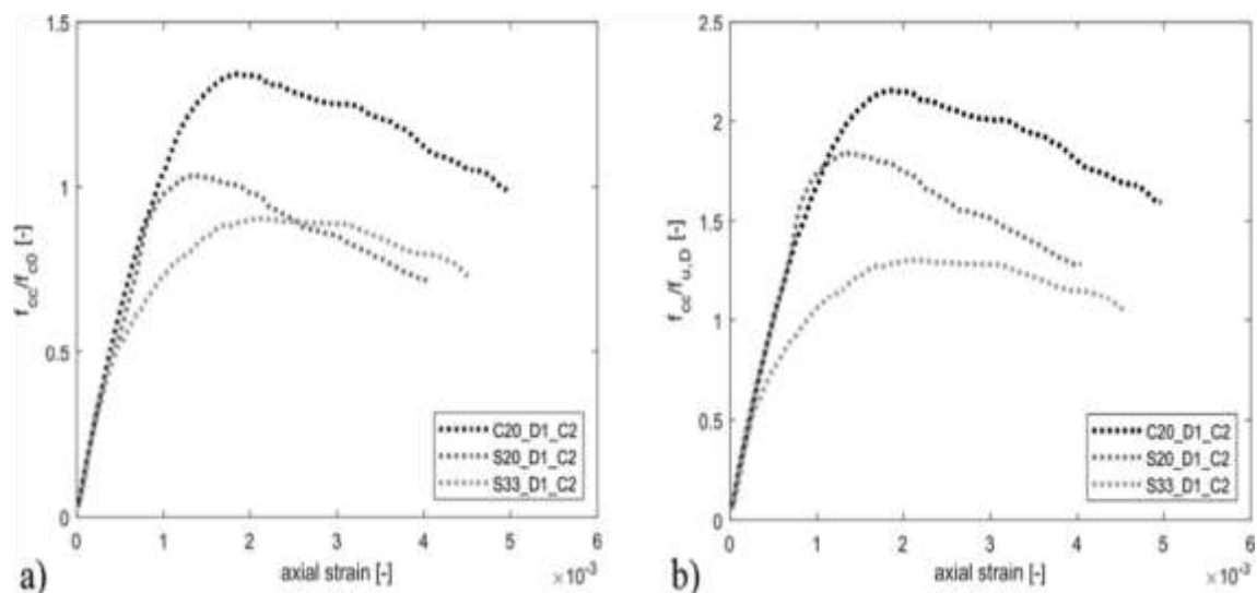
Fig. 9. Relative axial stress – strain curve with respect to the undamaged cases (a) and to the residual axial capacity of the damaged specimens ( b ).
