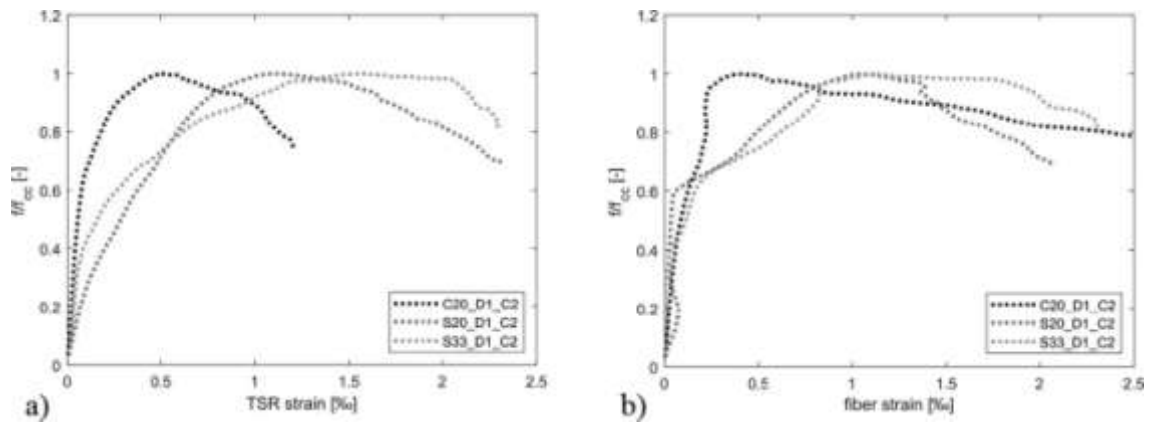
Fig. 11. TSR (a) and fiber (b) strains in the damaged repaired specimens.
