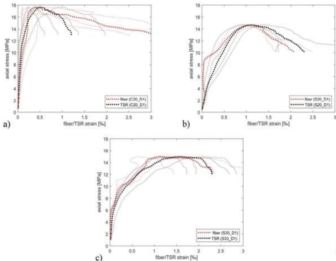
Fig. 8. Axial stress – fiber and TSR strain for damaged repaired specimens. a) C20_D1_C2, b) S20_D1_C2, c) S33_D1_C2.
