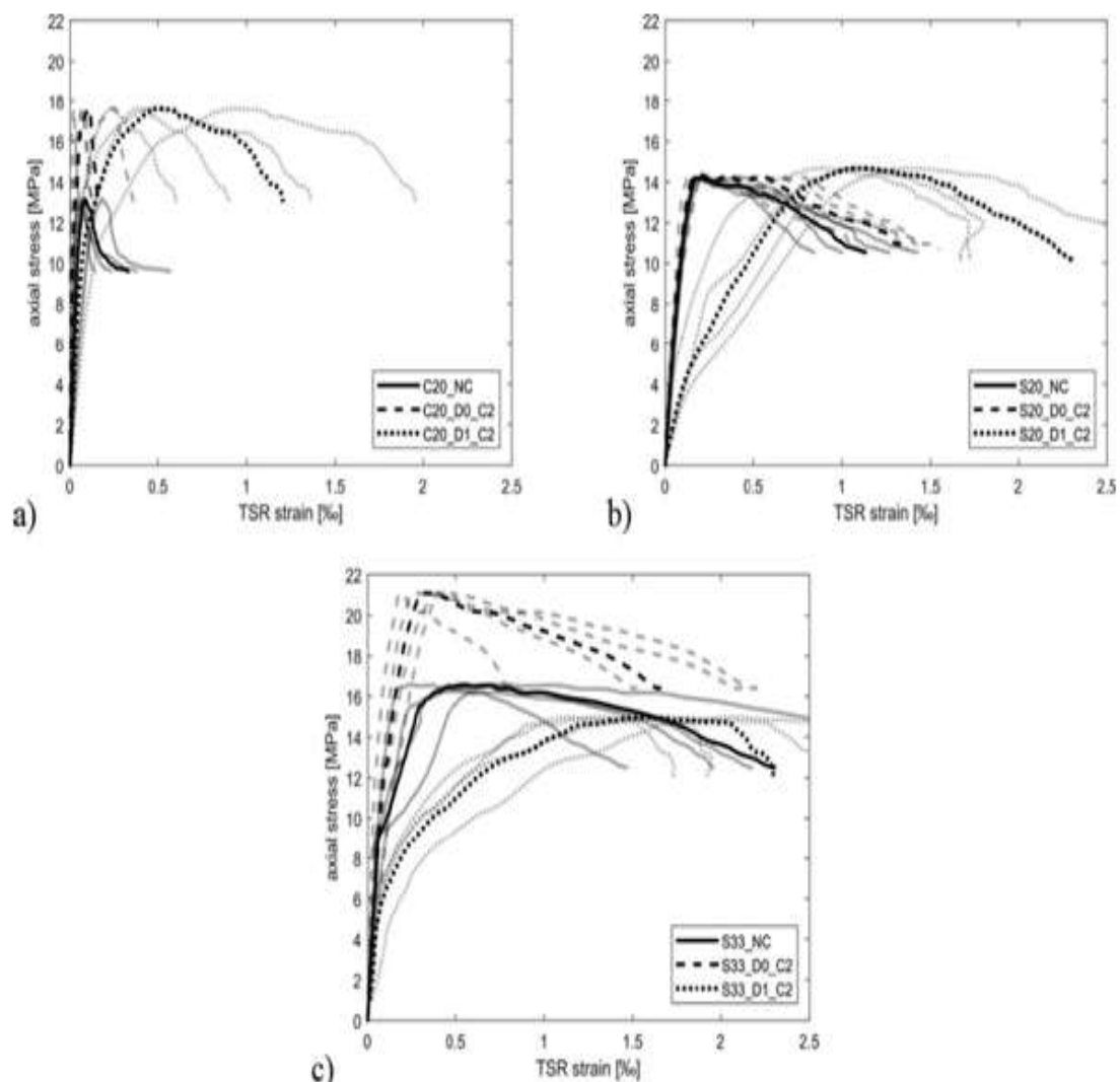
Fig. 7. Axial stress – TSR strains for unconfined, undamaged strengthened and damaged repaired columns. (a) C20, b) S20 and c) S_33 specimens.
