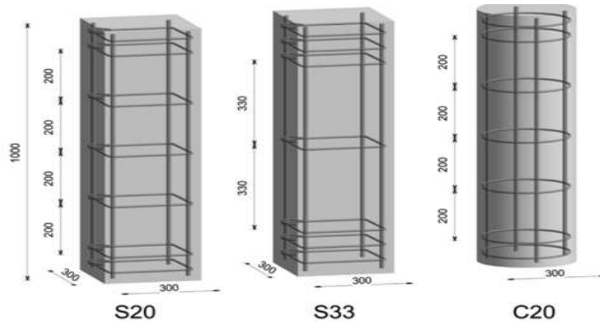
Fig. 1. Reinforcement details.
