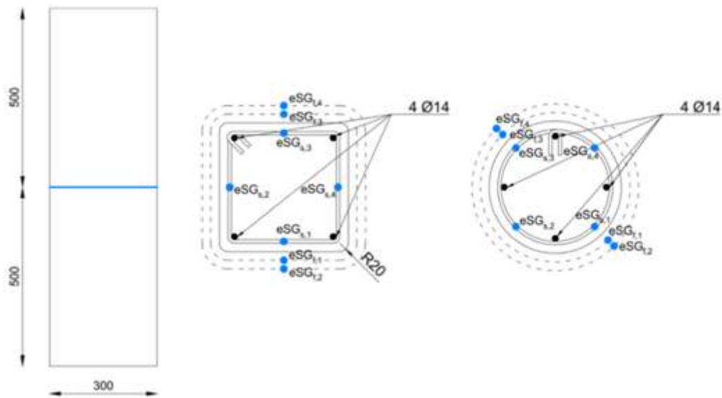
Fig. 2. Disposition of eSGs to evaluate stirrup and fibers strains.
