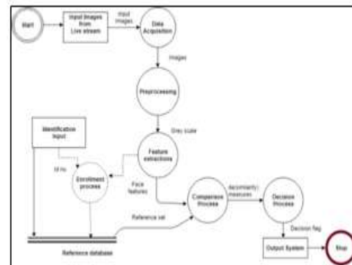
Fig 5: Flow of data in the system
