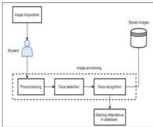
Fig 4: Activity Diagram of System
