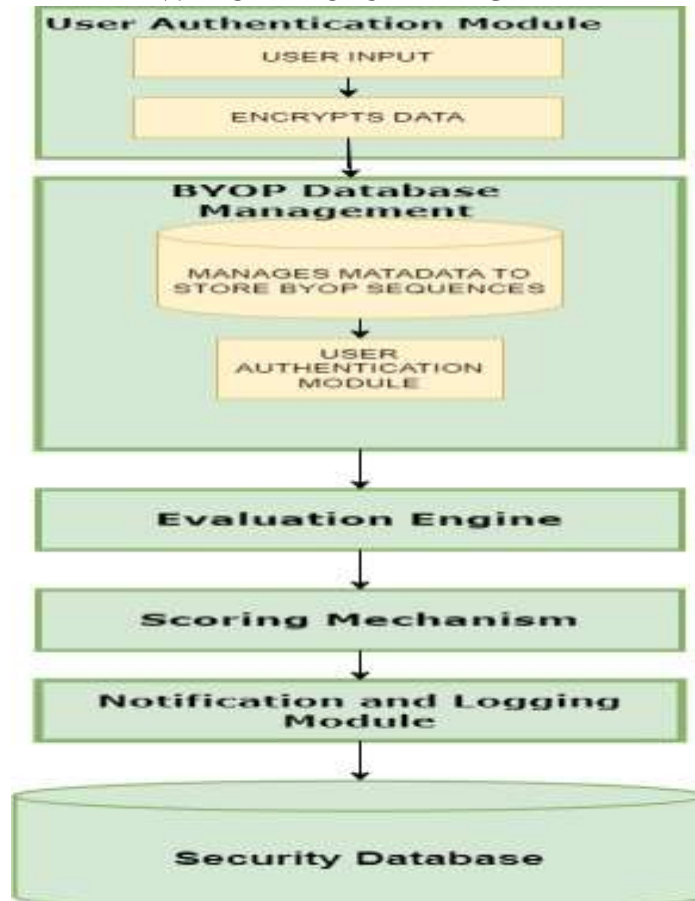
Fig:BYOP Software Puzzle Methodology: Architectural Overview
