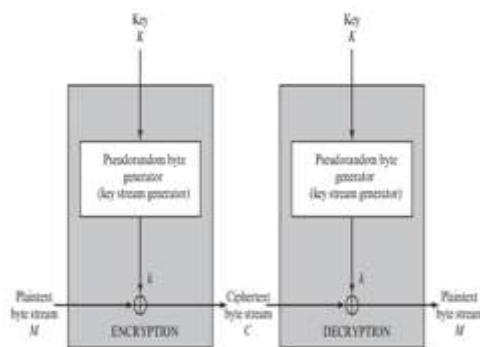
Fig.4. Stream Cipher
