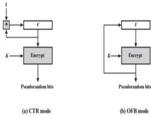
Fig.3. Block Cipher-Based PRNG Mechanisms
