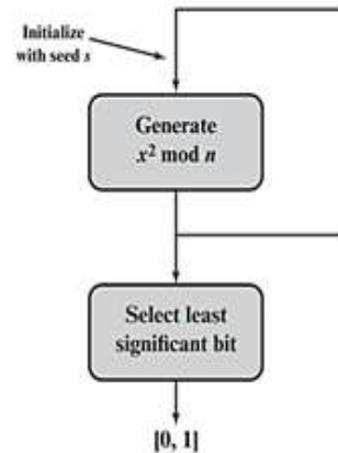
Fig.2. Blum Blum Shub Block Diagram
