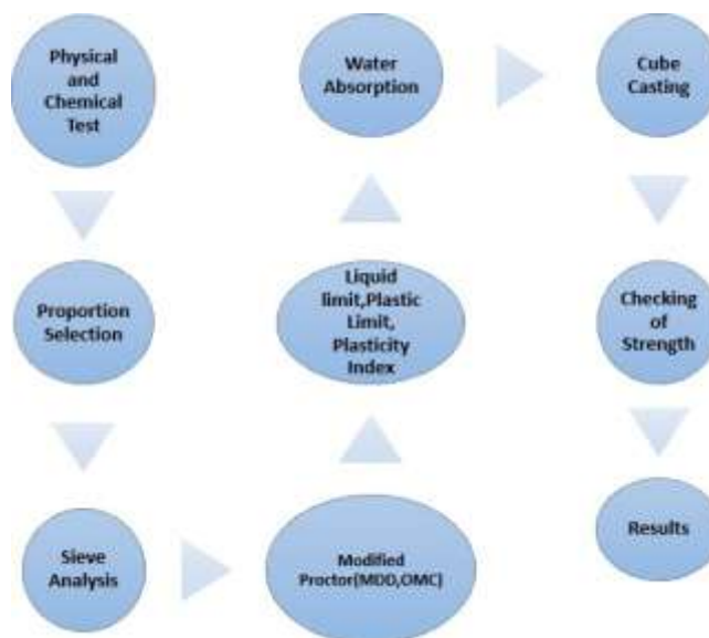
Fig -2: Process Cycle for CTB and CTSB
