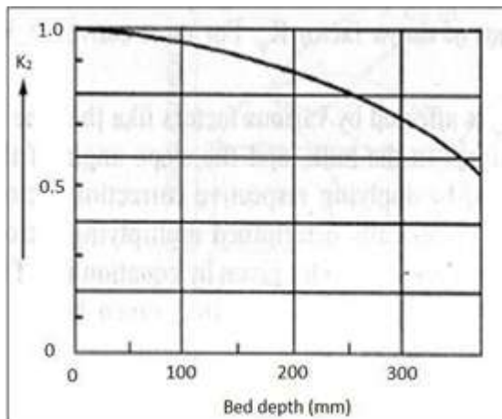
Fig -3: Graph of K_2 against Bed Depth
