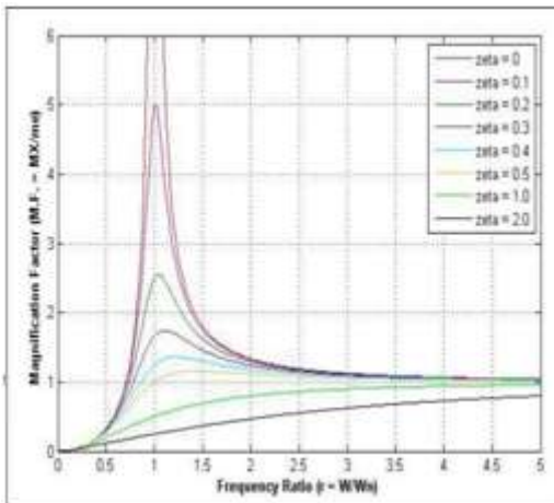
Fig – 6: Frequency Response of System Subjected to Centrifugal Force Type Excitation
