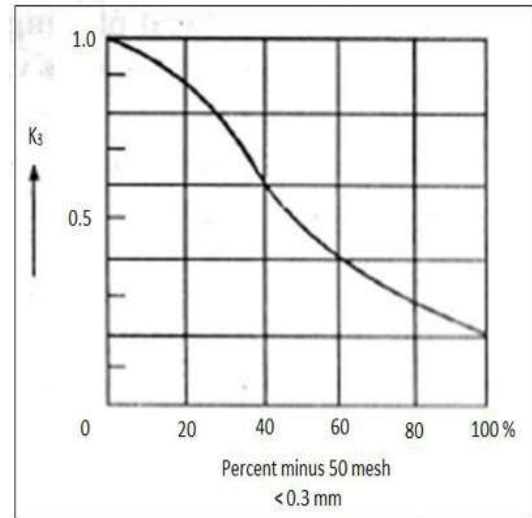
Fig - 4: Graph of K_3 against Percent Minus 50 Mesh
