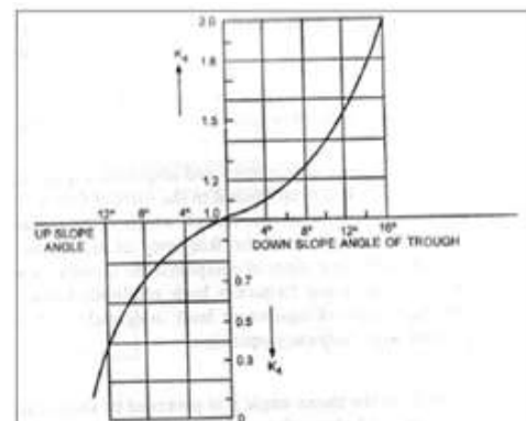
Fig - 5: Graph of K_4 against Slope Angle
