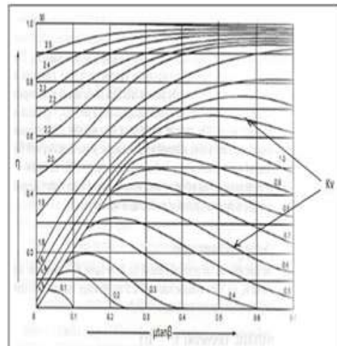
Fig – 2: Graph of Efficiency of Transport against \mu \tan \beta
