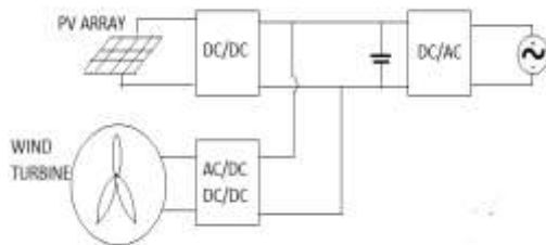
Figure 1: Hybrid grid basic structure
