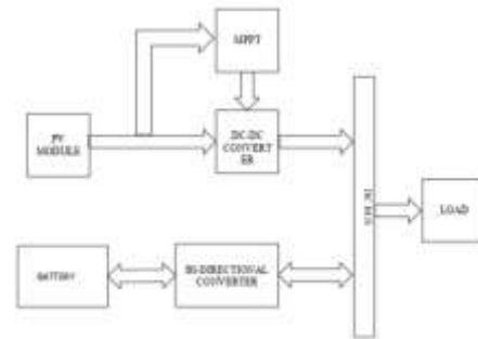
Figure 2: Overall block diagram of PV energy system
