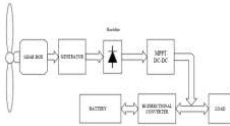
Figure 3: Wind turbine basic structure
