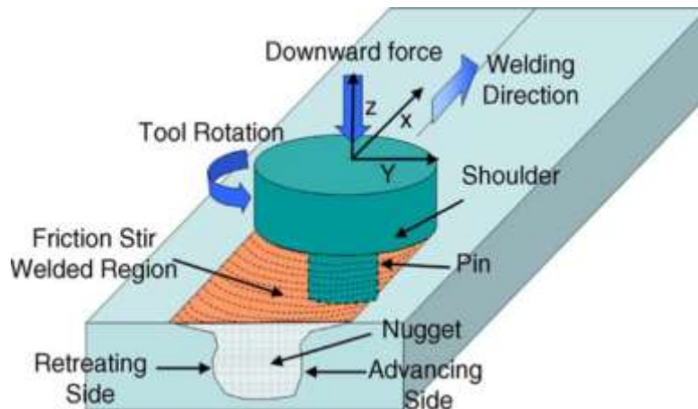
Figure 1. Schematic drawing of FSW
