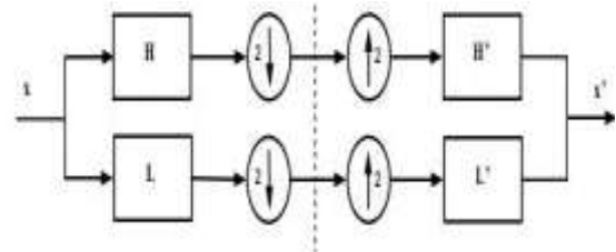
Fig. 4: Filter Bank Scheme for DWT
