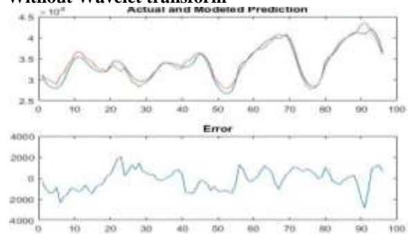
Fig. 11: Comparison between the predicted and actual load employing the proposed model using LM training without WT.
