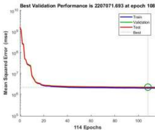
Fig. 13: Neural network performance during training, testing & validation without WT.
