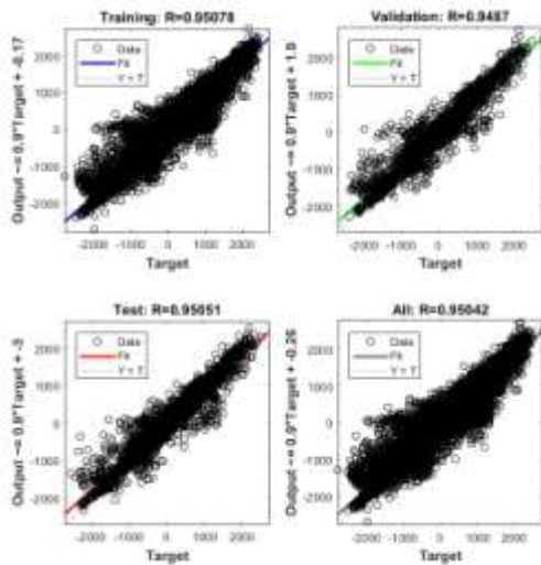
Fig. 9: Regression plot during training, testing & validation for Proposed Levenberg-Marquardt (LM) training algorithm with WT.
