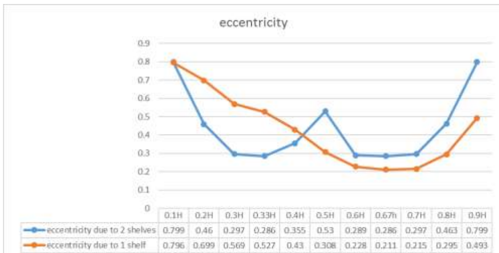
Fig. 6. eccentric behavior of wall with respect to location of shelf/shelves
