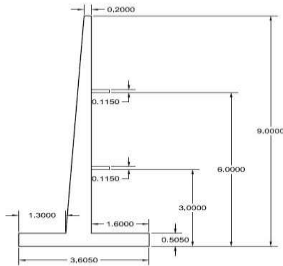
Fig. 3. retaining wall with two shelves
