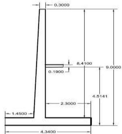
Fig.2.Retaining wall with one relief shelf
