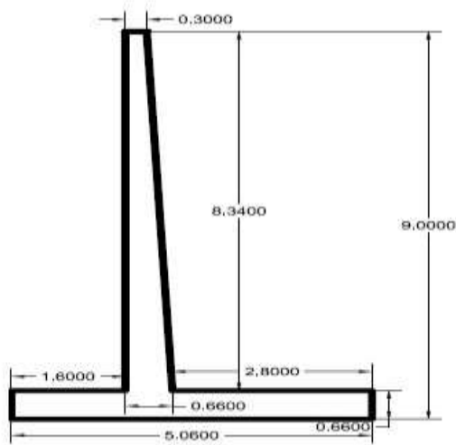
Fig.1.Cantilever retaining wall
