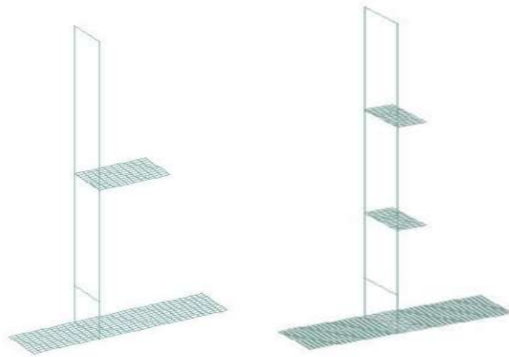
Figure 4 STAAD model for wall with 1 shelf and two shelves
