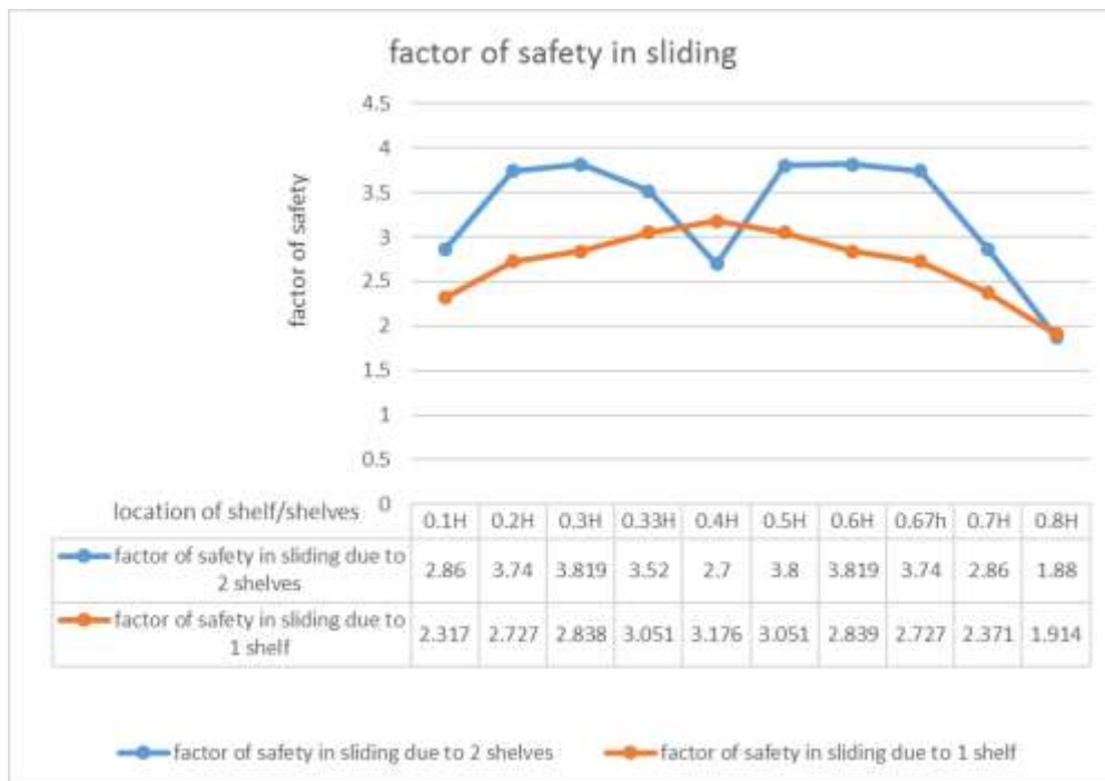
Fig. 7. factor of safety in sliding against location of shelf/shelves
