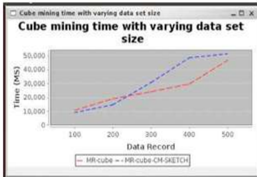
Figure.4 Cube mining time with vary in dataset size.
