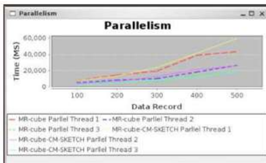
Figure.5 Parallelism in twitter dataset.
