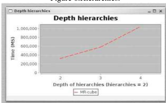
Figure.7 Map Reduce Depth hierarchies.
