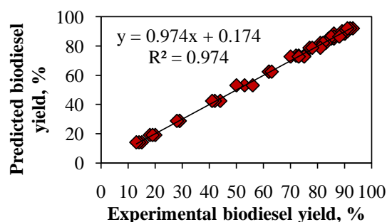
Figure 1. Correlation between predicted and experimental biodiesel yield
