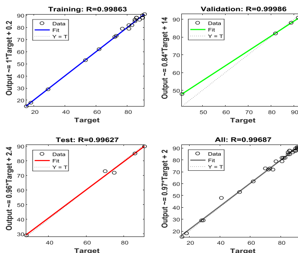
Figure 2. Correlation between ANN predicted biodiesel yield and experimental biodiesel yield for 30 runs
