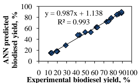
Figure 3. Correlation between ANN predicted biodiesel yield and experimental biodiesel yield for 18 runs
