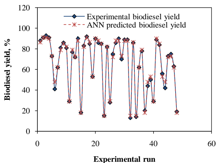
Figure 4. ANN model prediction performance for 48 runs
