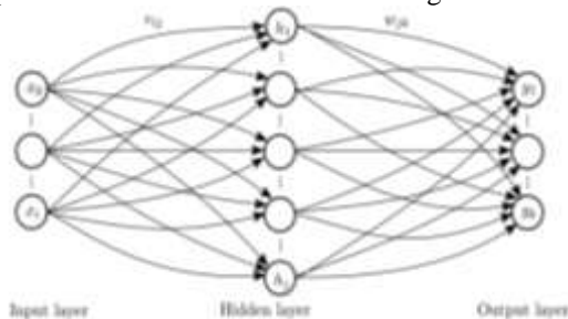
Figure 2: Basic Structure of a Multilayer Artificial Neuron.
