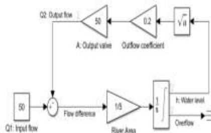
Figure 4: Simulink Model of the River
