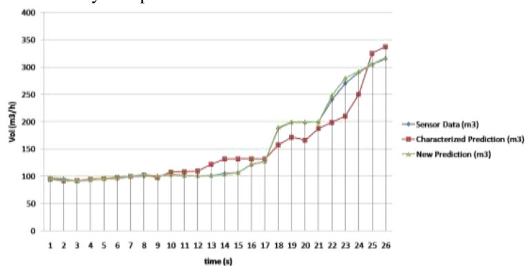
Figure 22: Comparative Flood Level Prediction Performance
