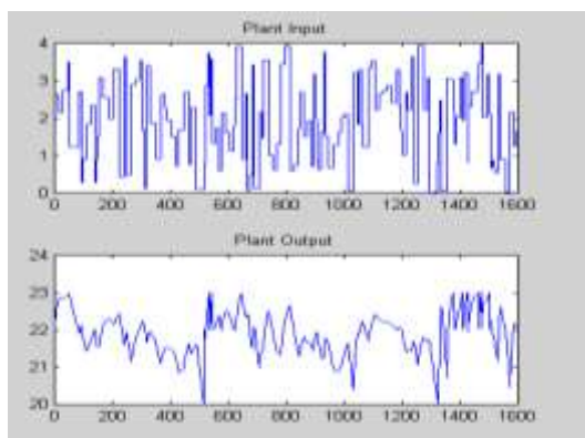
Figure 10: System Identification with ANN
