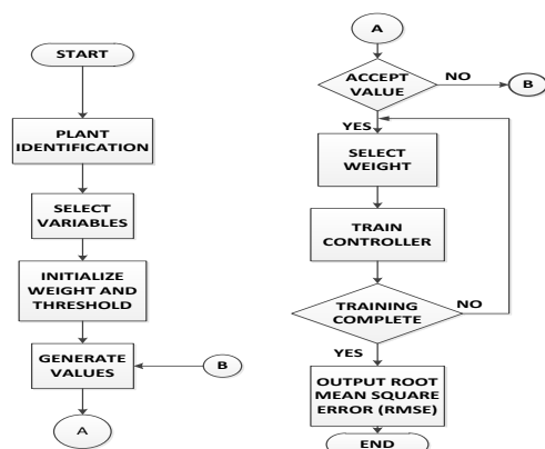
Figure9: Flowchart for ANN Training
