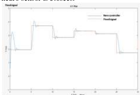
Figure 14: Step Response of the Neuro Controller
