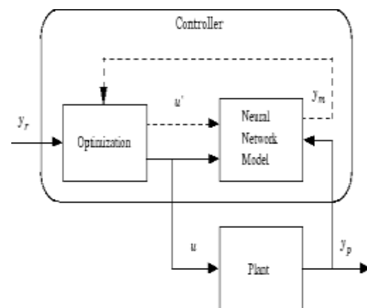
Figure 11: Block Diagram of the Neuro Controller
