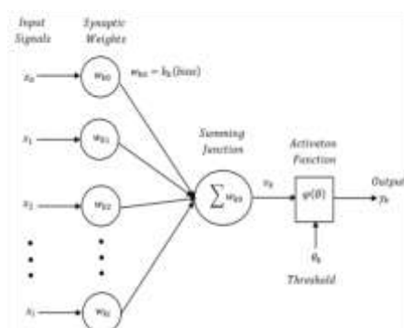
Figure 1: Model Description of an Artificial Neuron
