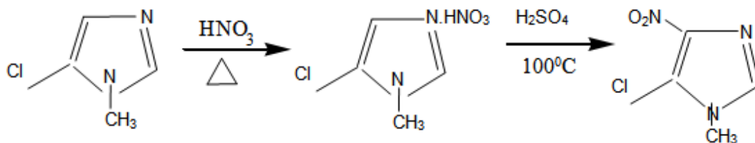
Figure 4.3: Synthesis of 1-Methyl, 4-nitro-5-chloroimidazole.
