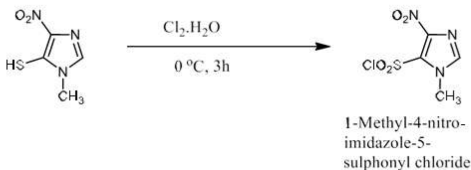
Figure 4.5: Synthesis of 1-Methyl-4-Nitro-Imidazole-5-Sulphonyl Chloride
