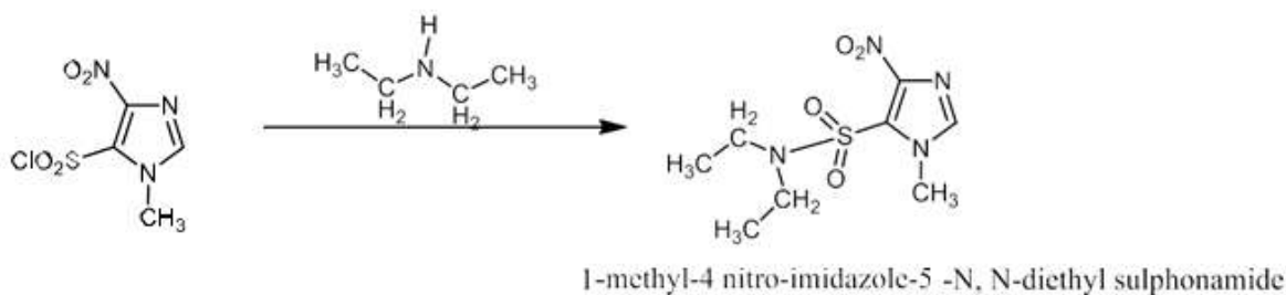
Figure 4.6: Synthesis of 1-methyl-4-nitro-imidazole-5-N, N-diethylsulphonamide
