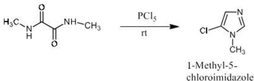
Figure 4.2: Synthesis of 1-Methyl-5-Chloroimidazole
