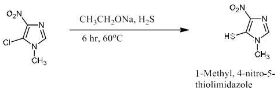
Figure 4.4 Synthesis of 1-Methyl, 4-nitro-5-thiolimidazole
